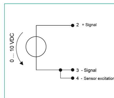
Transmitter connection
